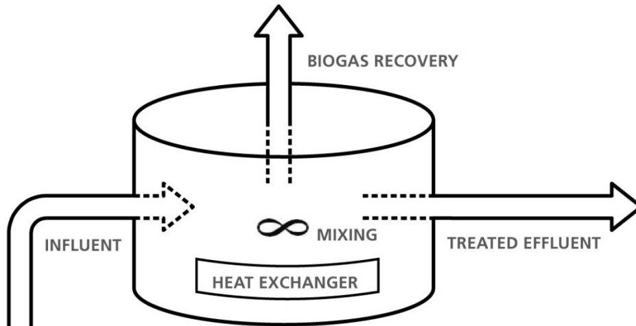
Figure 3 – Simplified complete mix digester schematic
