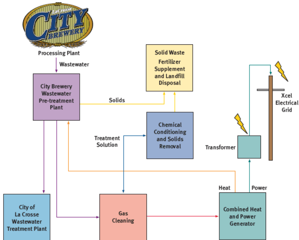
Figure 12 – Process flow chart for Gundersen Lutheran and City Brewing Company. Graphic courtesy of Gundersen Lutheran.
