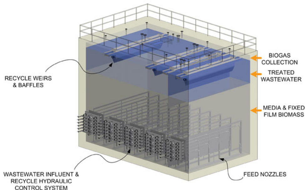
Figure 18 - MFT Digester Schematic. Graphic courtesy of Ecolab.
