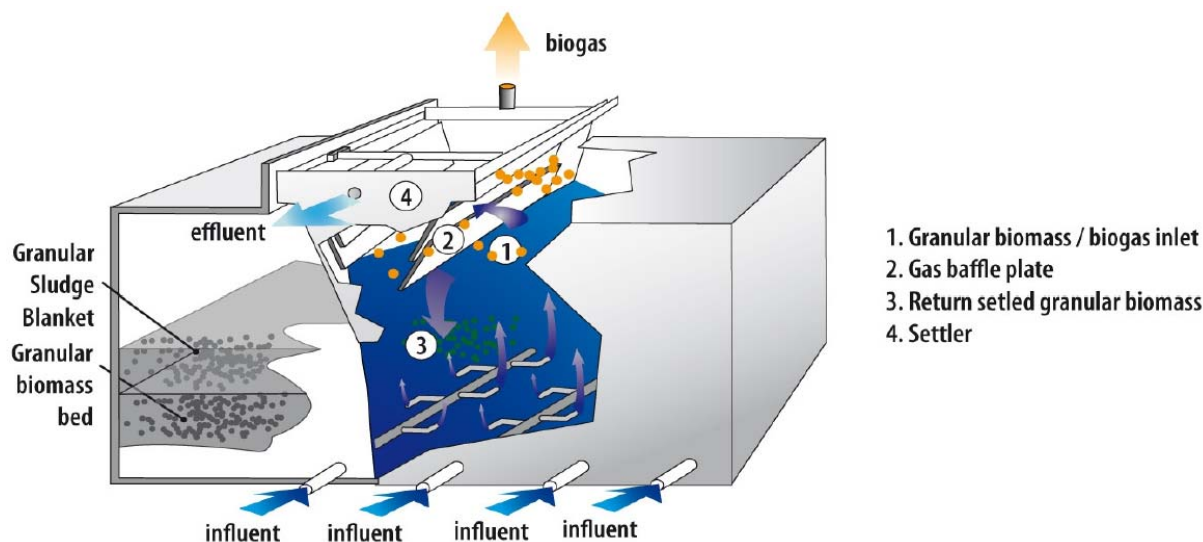
Figure 8 - UASB Concept Schematic. Graphic courtesy of Richard Mattocks, Biothane, Veolia Water, Inc.
