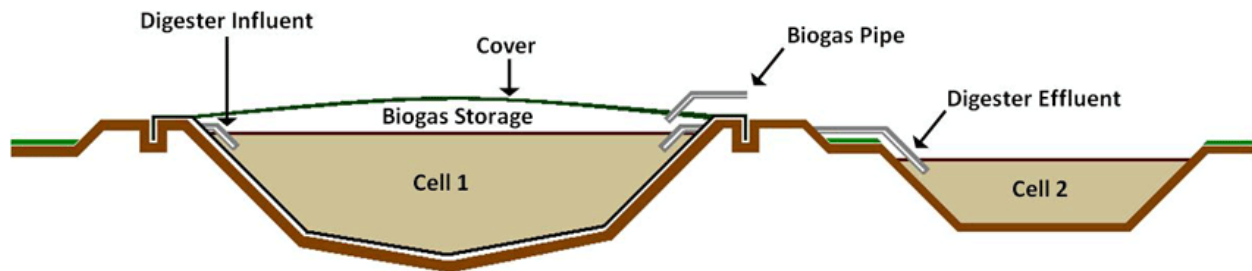
Figure 2 - Covered lagoon schematic. Graphic courtesy of US EPA AgSTAR Program.
