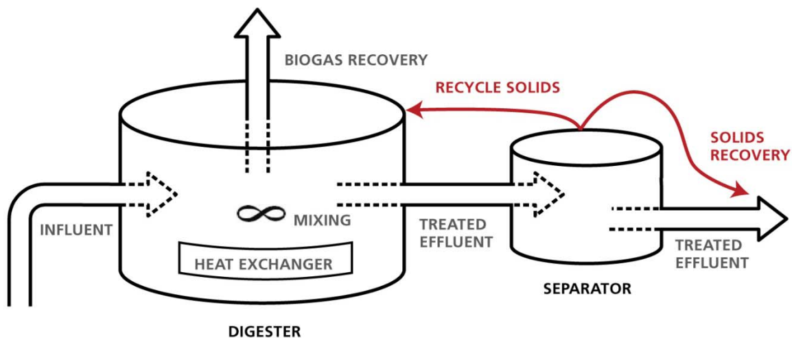
Figure 4 - Simplified anaerobic contact process schematic
