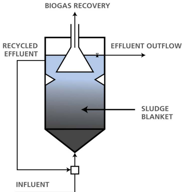
Figure 5 - Upflow anaerobic sludge blanket digester. Graphic courtesy of Doug Hamilton Oklahoma State University
